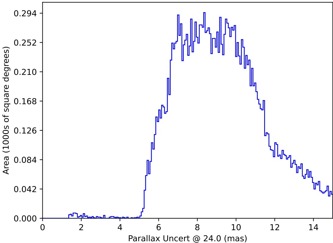
uniform_u_expt38_nscale1.1v3.4_10yrs : Parallax Uncert @ 24.0
