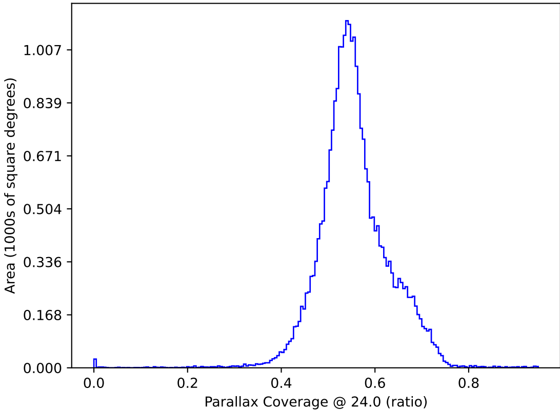
uniform_u_expt38_nscale1.1v3.4_10yrs : Parallax Coverage @ 24.0
