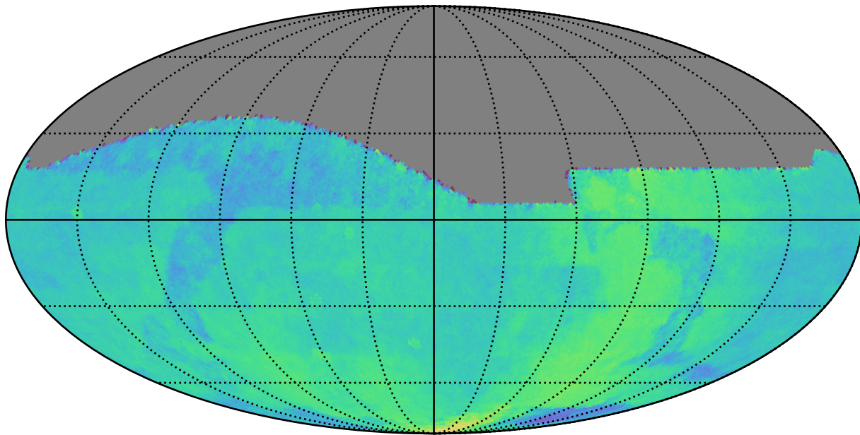
uniform_u_expt38_nscale1.1v3.4_10yrs : Parallax Coverage @ 22.4
