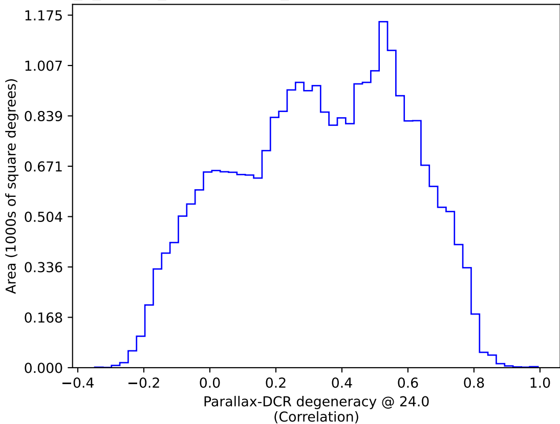
uniform_u_expt38_nscale1.1v3.4_10yrs : Parallax-DCR degeneracy @ 24.0
