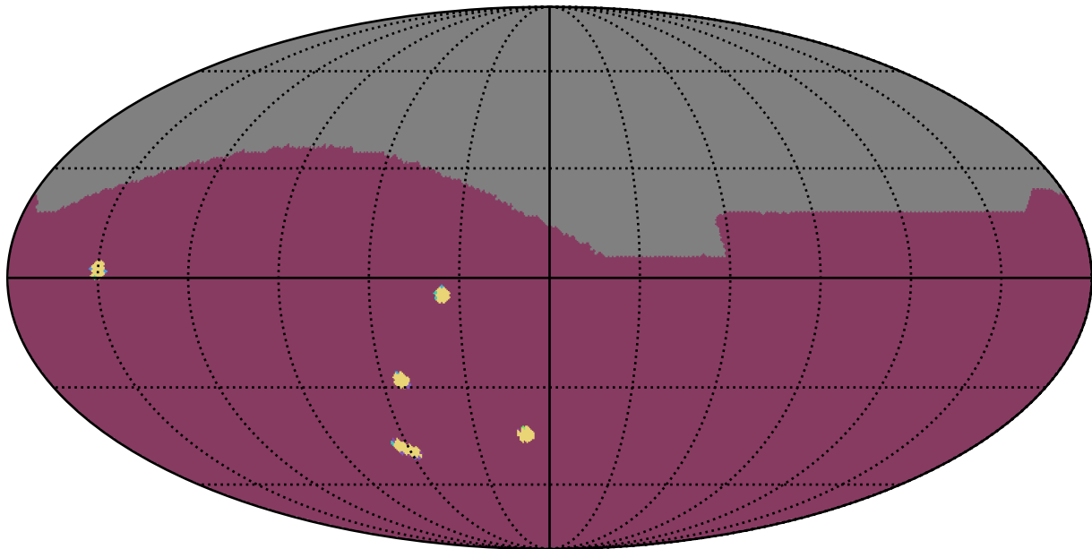
uniform_u_expt38_nscale1.1v3.4_10yrs : NumberOfQuickRevisits
