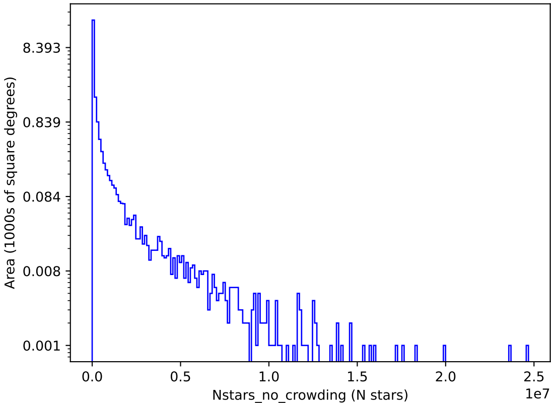
uniform_u_expt38_nscale1.1v3.4_10yrs y: Nstars_no_crowding
