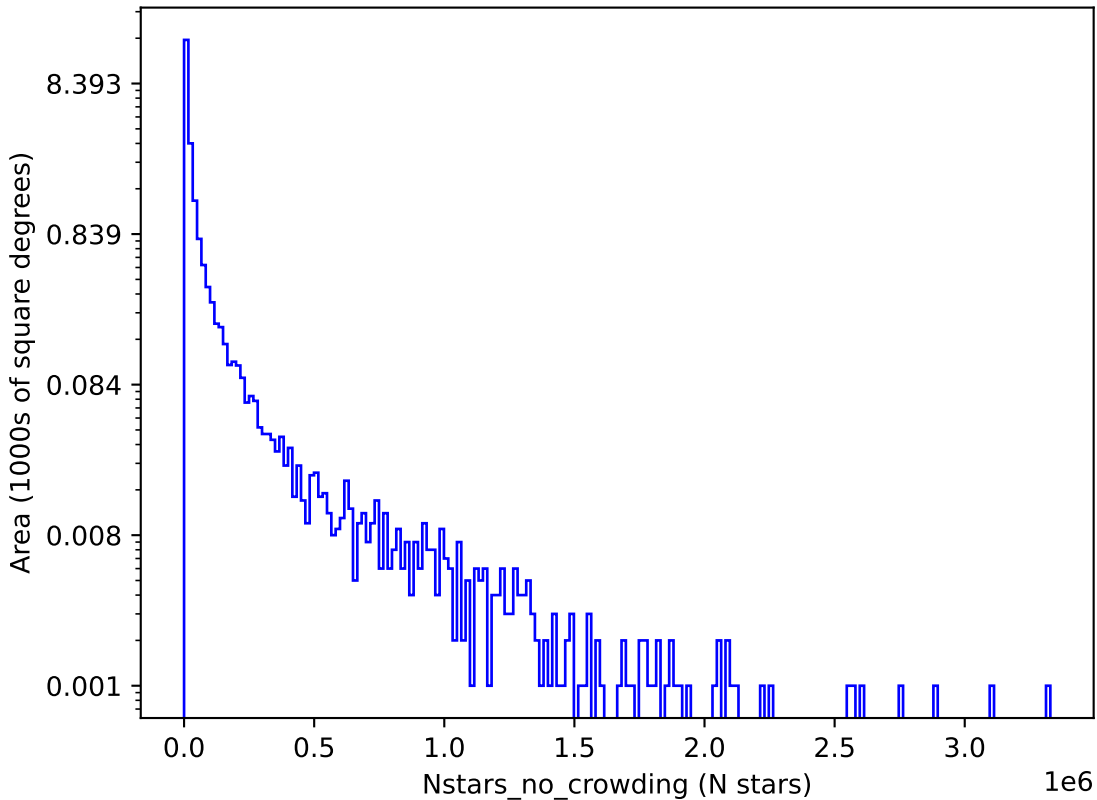
uniform_u_expt38_nscale1.1v3.4_10yrs u: Nstars_no_crowding
