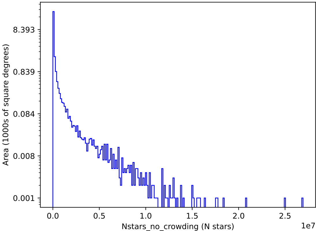
uniform_u_expt38_nscale1.1v3.4_10yrs i: Nstars_no_crowding
