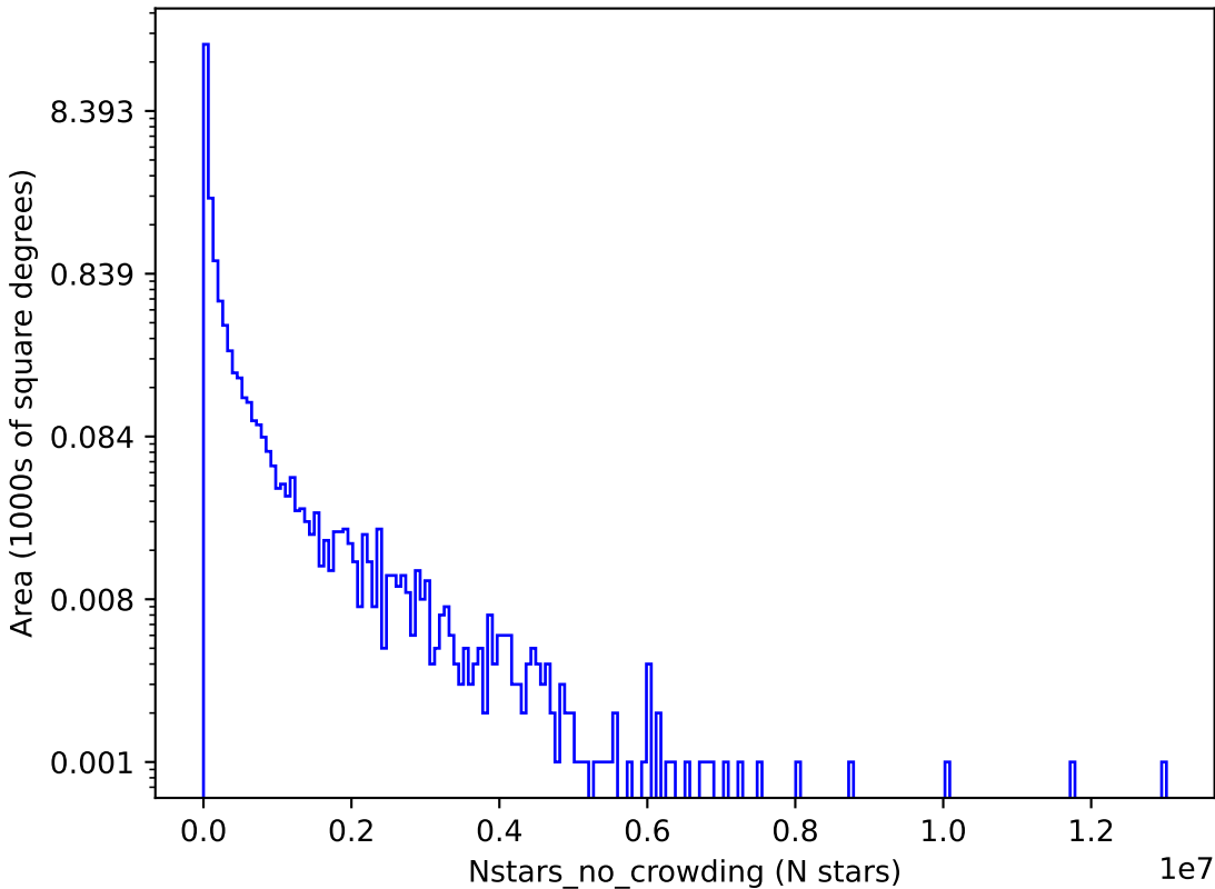
uniform_u_expt38_nscale1.1v3.4_10yrs g: Nstars_no_crowding
