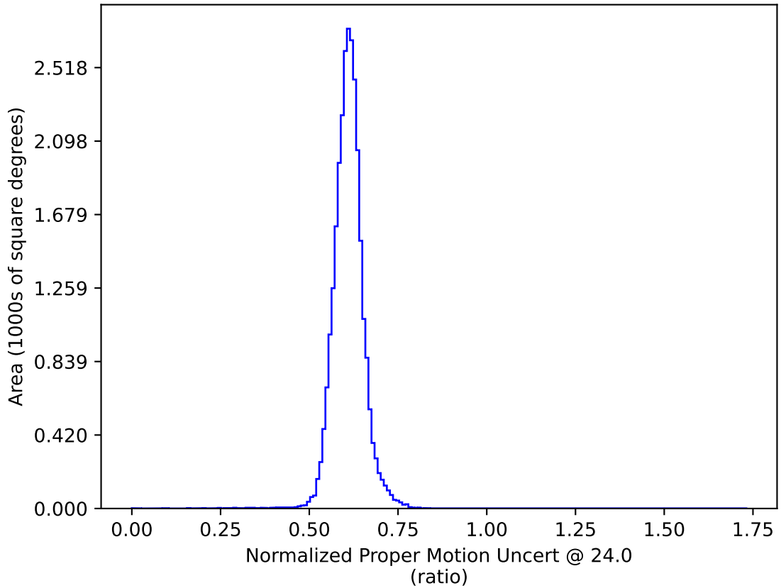
uniform_u_expt38_nscale1.1v3.4_10yrs : Normalized Proper Motion Uncert @ 24.0
