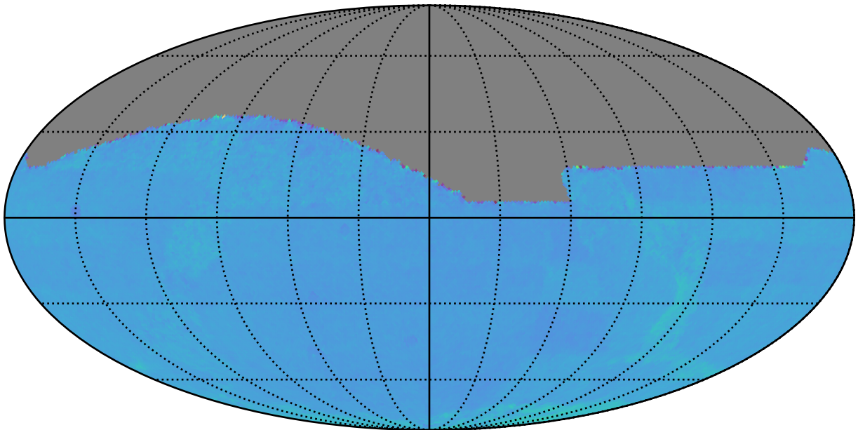
uniform_u_expt38_nscale1.1v3.4_10yrs : Normalized Proper Motion Uncert @ 20.5
