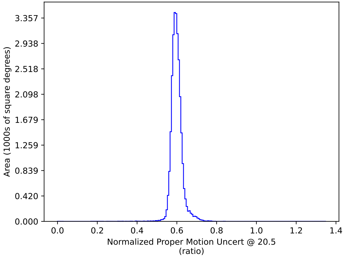
uniform_u_expt38_nscale1.1v3.4_10yrs : Normalized Proper Motion Uncert @ 20.5
