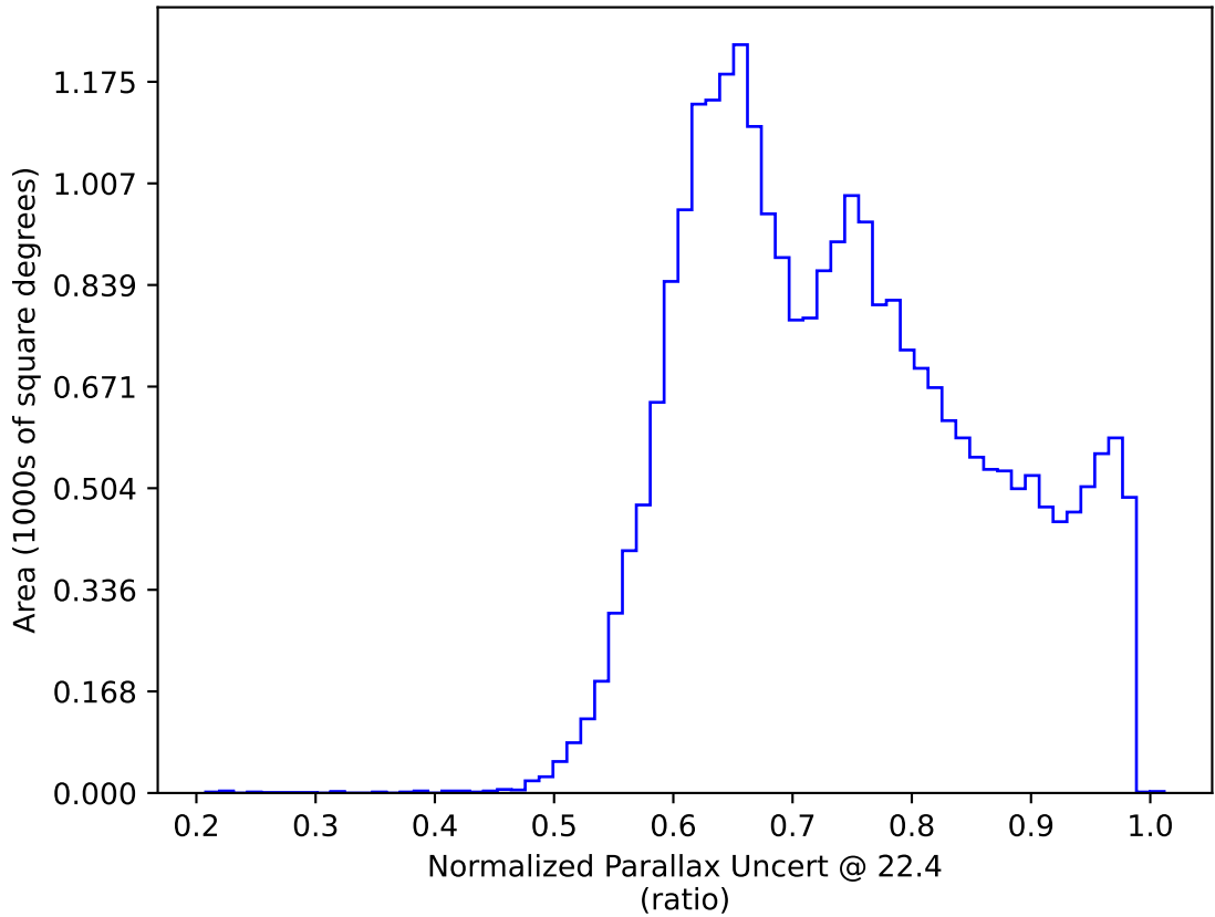
uniform_u_expt38_nscale1.1v3.4_10yrs : Normalized Parallax Uncert @ 22.4
