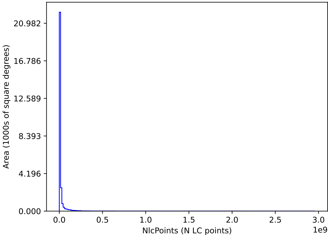
uniform_u_expt38_nscale1.1v3.4_10yrs : NlcPoints
