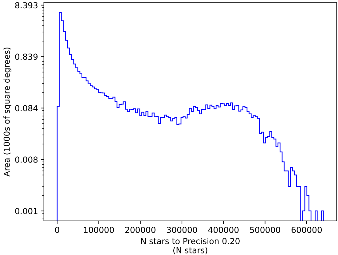
uniform_u_expt38_nscale1.1v3.4_10yrs z: N stars to Precision 0.20
