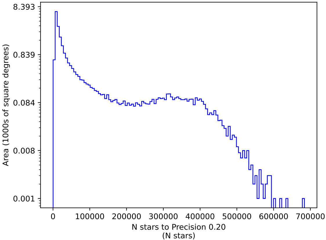
uniform_u_expt38_nscale1.1v3.4_10yrs y: N stars to Precision 0.20
