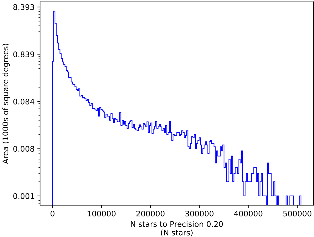
uniform_u_expt38_nscale1.1v3.4_10yrs u: N stars to Precision 0.20
