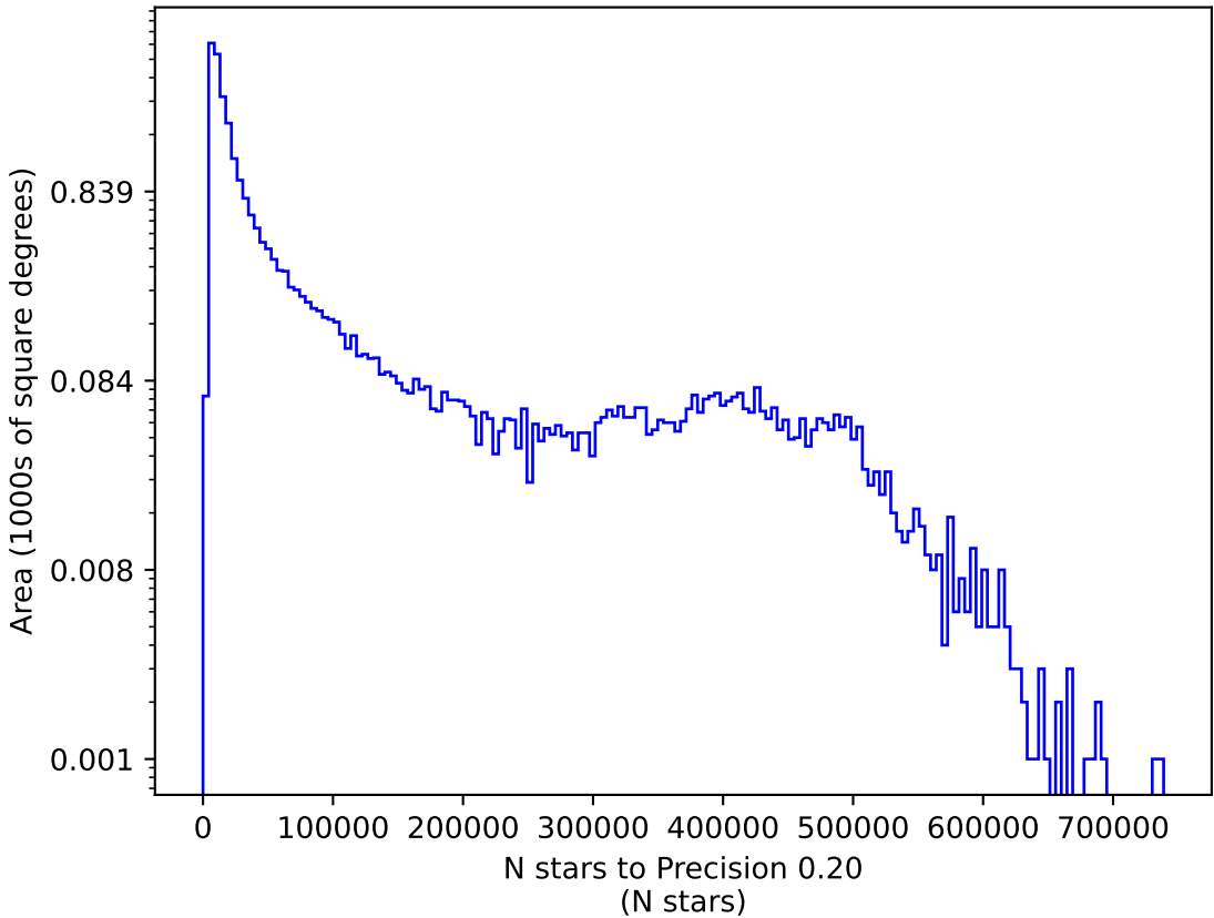
uniform_u_expt38_nscale1.1v3.4_10yrs r: N stars to Precision 0.20
