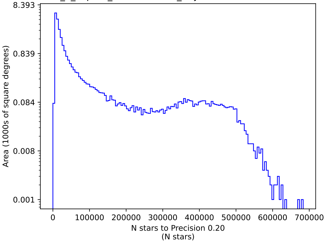
uniform_u_expt38_nscale1.1v3.4_10yrs i: N stars to Precision 0.20
