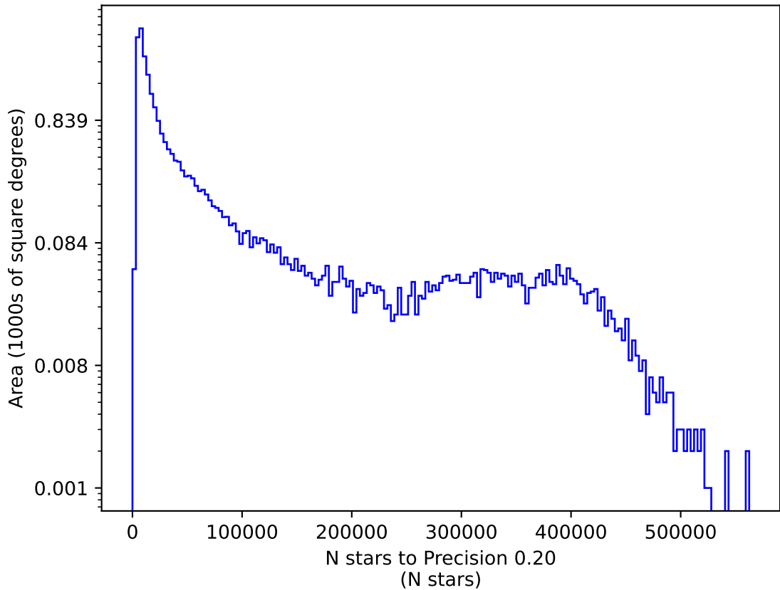
uniform_u_expt38_nscale1.1v3.4_10yrs g: N stars to Precision 0.20
