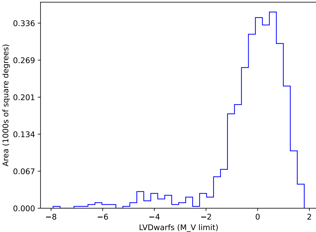
uniform_u_expt38_nscale1.1v3.4_10yrs gi SCP: LVDwarfs
