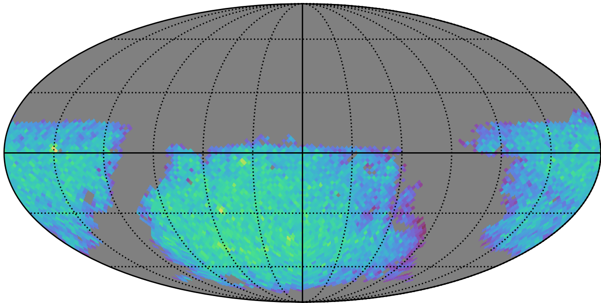
uniform_u_expt38_nscale1.1v3.4_10yrs gi: LVDwarfs
