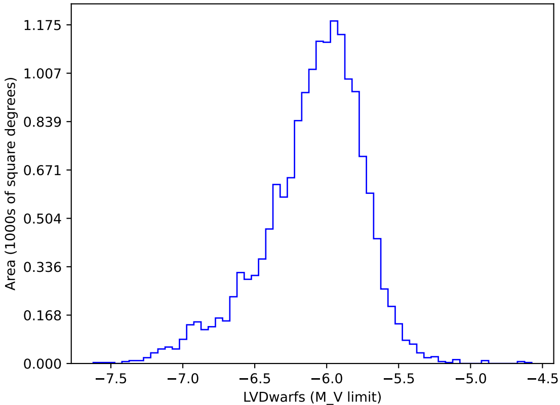
uniform_u_expt38_nscale1.1v3.4_10yrs gi: LVDwarfs
