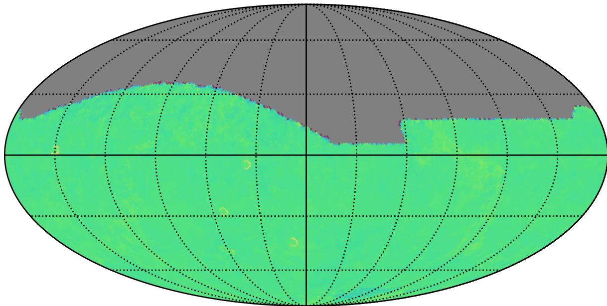
uniform_u_expt38_nscale1.1v3.4_10yrs z: Kuiper rotTelPos
