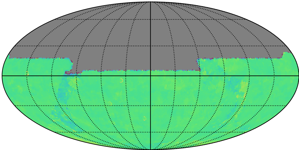
uniform_u_expt38_nscale1.1v3.4_10yrs u: Kuiper rotTelPos
