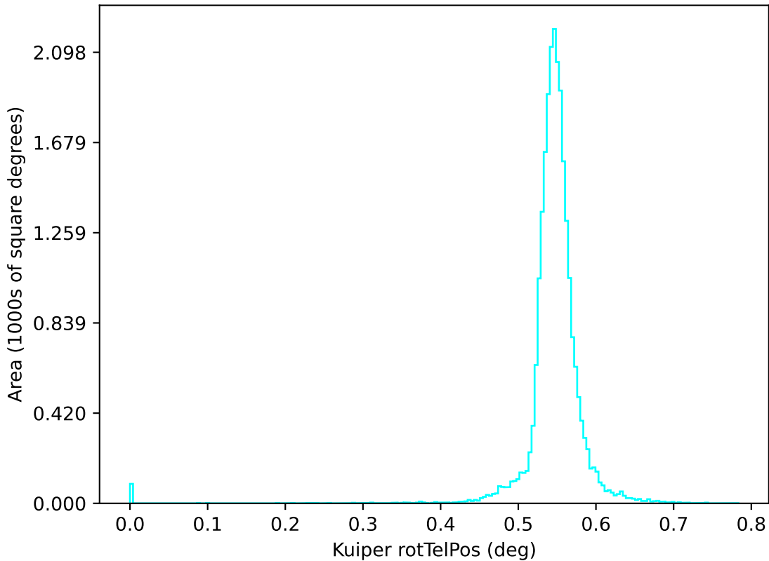
uniform_u_expt38_nscale1.1v3.4_10yrs u: Kuiper rotTelPos
