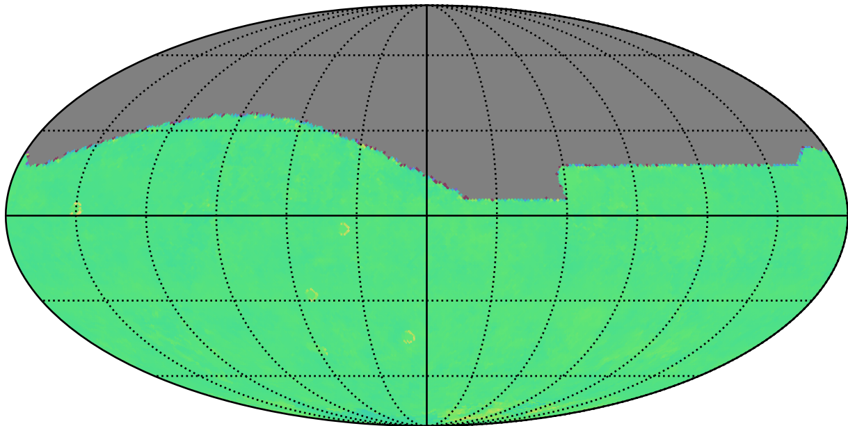
uniform_u_expt38_nscale1.1v3.4_10yrs r: Kuiper rotTelPos
