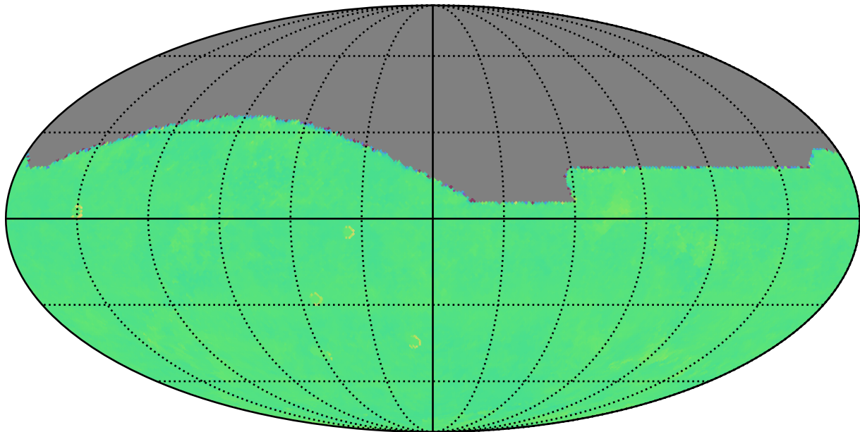
uniform_u_expt38_nscale1.1v3.4_10yrs i: Kuiper rotTelPos
