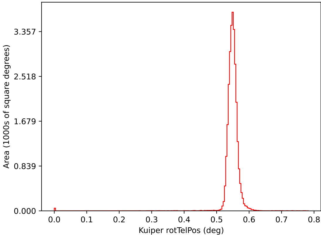
uniform_u_expt38_nscale1.1v3.4_10yrs i: Kuiper rotTelPos
