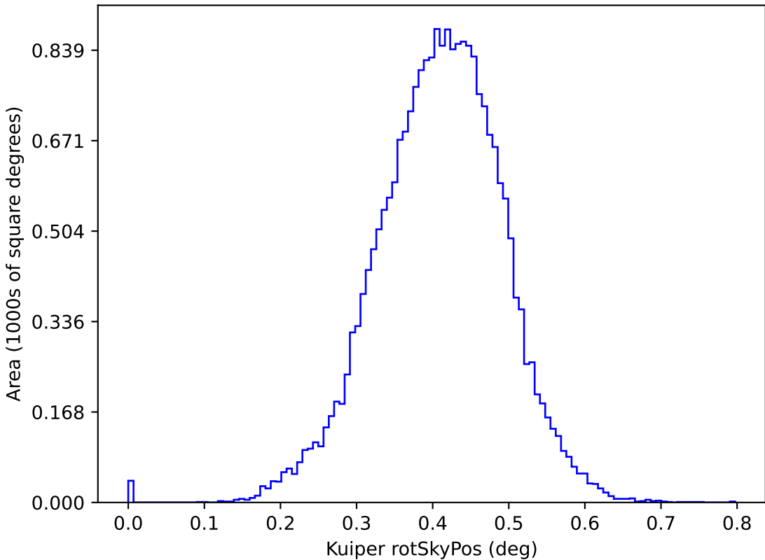
uniform_u_expt38_nscale1.1v3.4_10yrs y: Kuiper rotSkyPos
