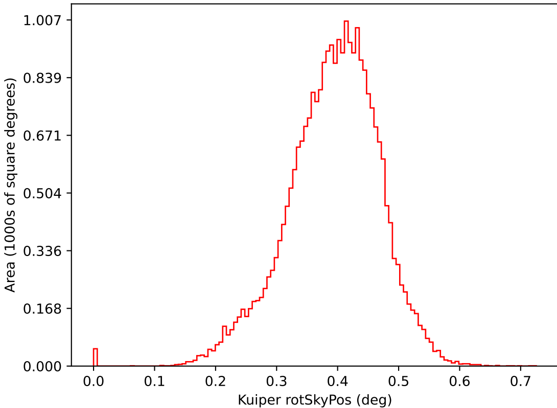
uniform_u_expt38_nscale1.1v3.4_10yrs i: Kuiper rotSkyPos
