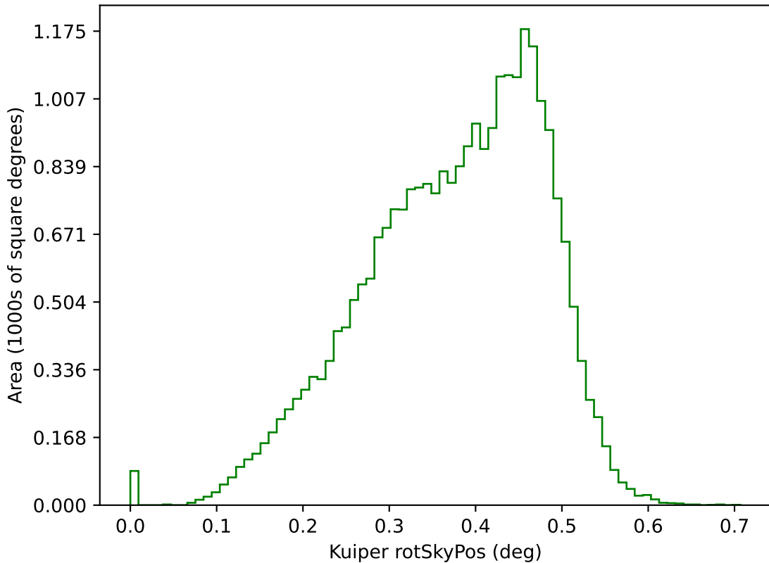
uniform_u_expt38_nscale1.1v3.4_10yrs g: Kuiper rotSkyPos
