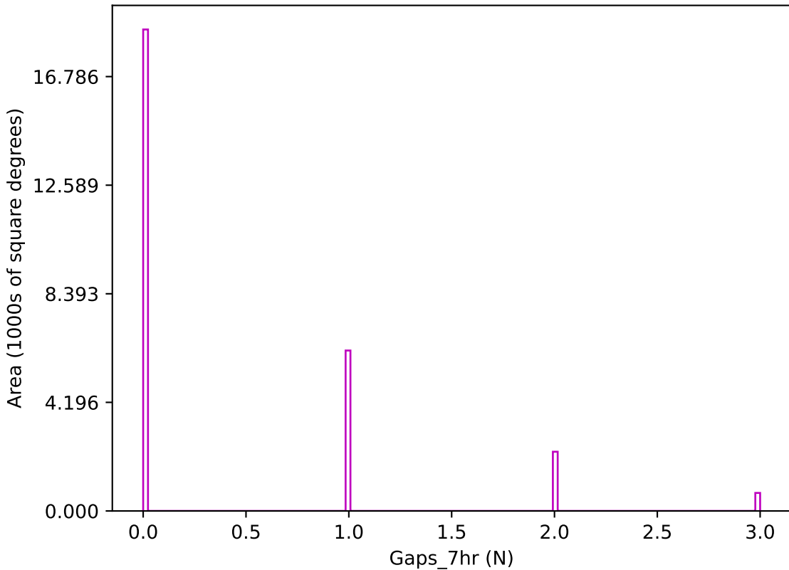
uniform_u_expt38_nscale1.1v3.4_10yrs z band: Gaps_7hr
