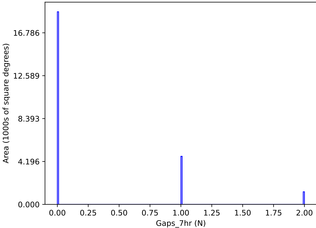
uniform_u_expt38_nscale1.1v3.4_10yrs y band: Gaps_7hr
