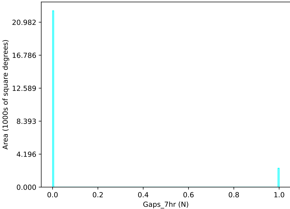
uniform_u_expt38_nscale1.1v3.4_10yrs u band: Gaps_7hr
