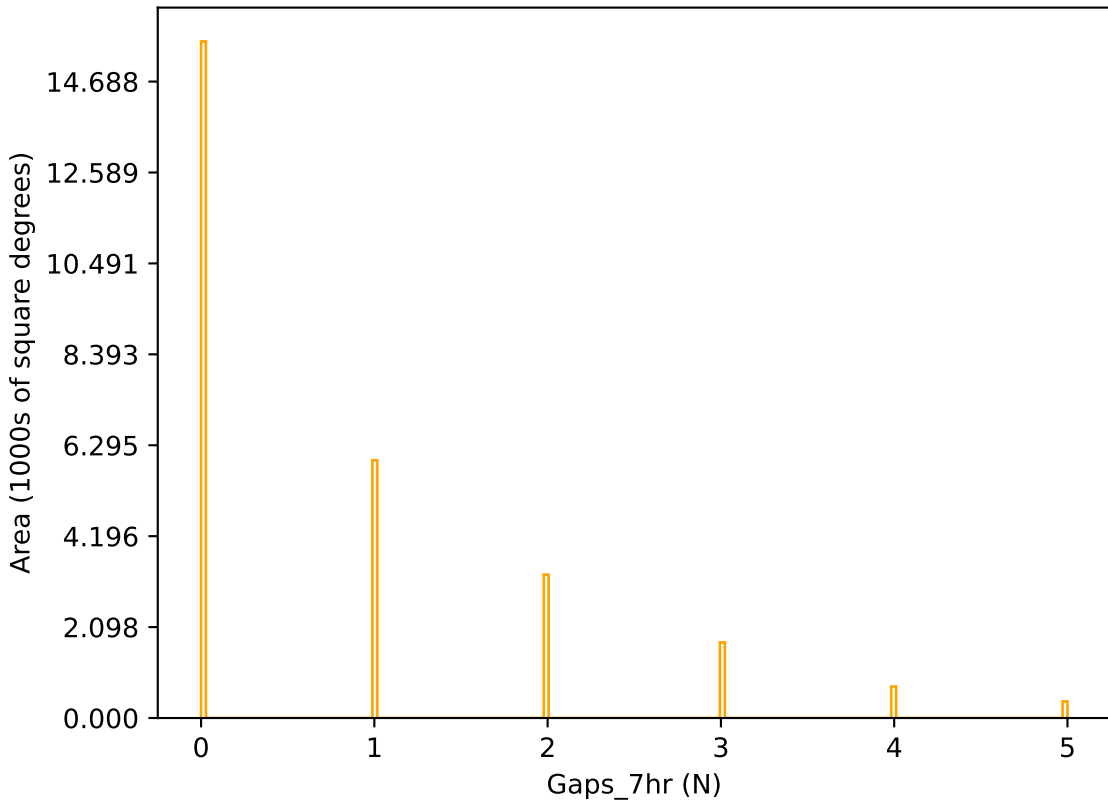
uniform_u_expt38_nscale1.1v3.4_10yrs r band: Gaps_7hr
