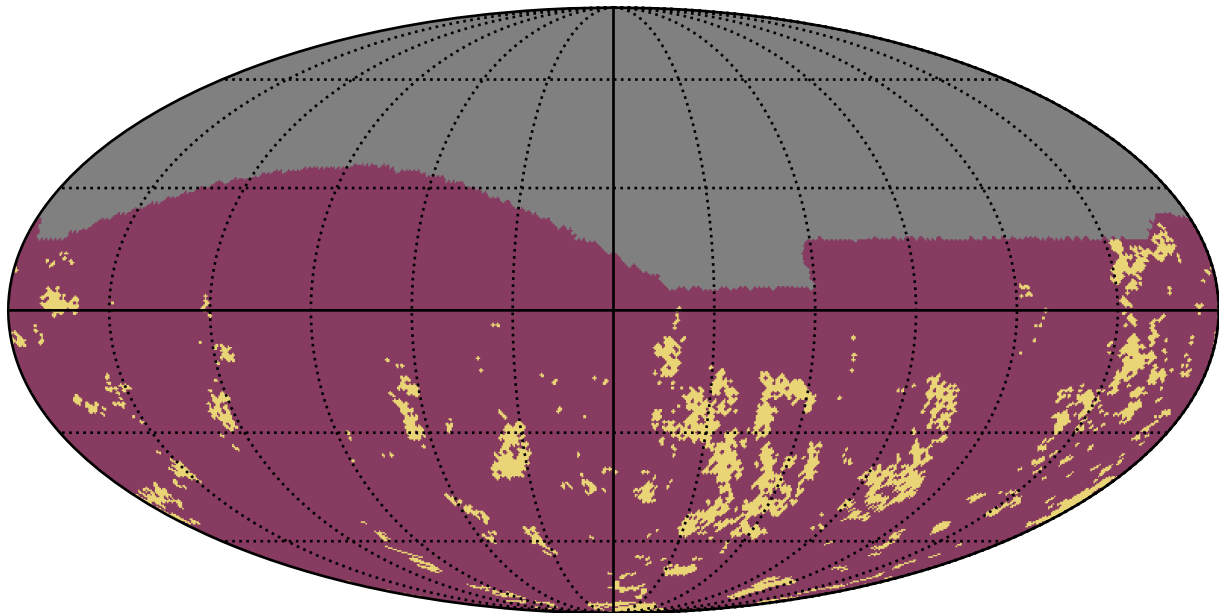
uniform_u_expt38_nscale1.1v3.4_10yrs g band: Gaps_7hr
