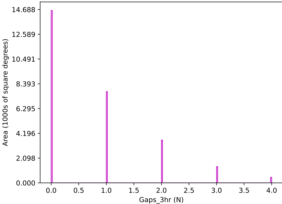
uniform_u_expt38_nscale1.1v3.4_10yrs z band: Gaps_3hr
