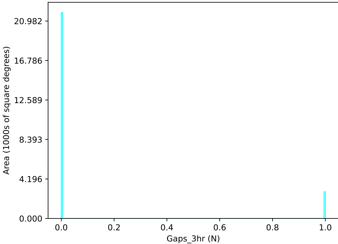
uniform_u_expt38_nscale1.1v3.4_10yrs u band: Gaps_3hr
