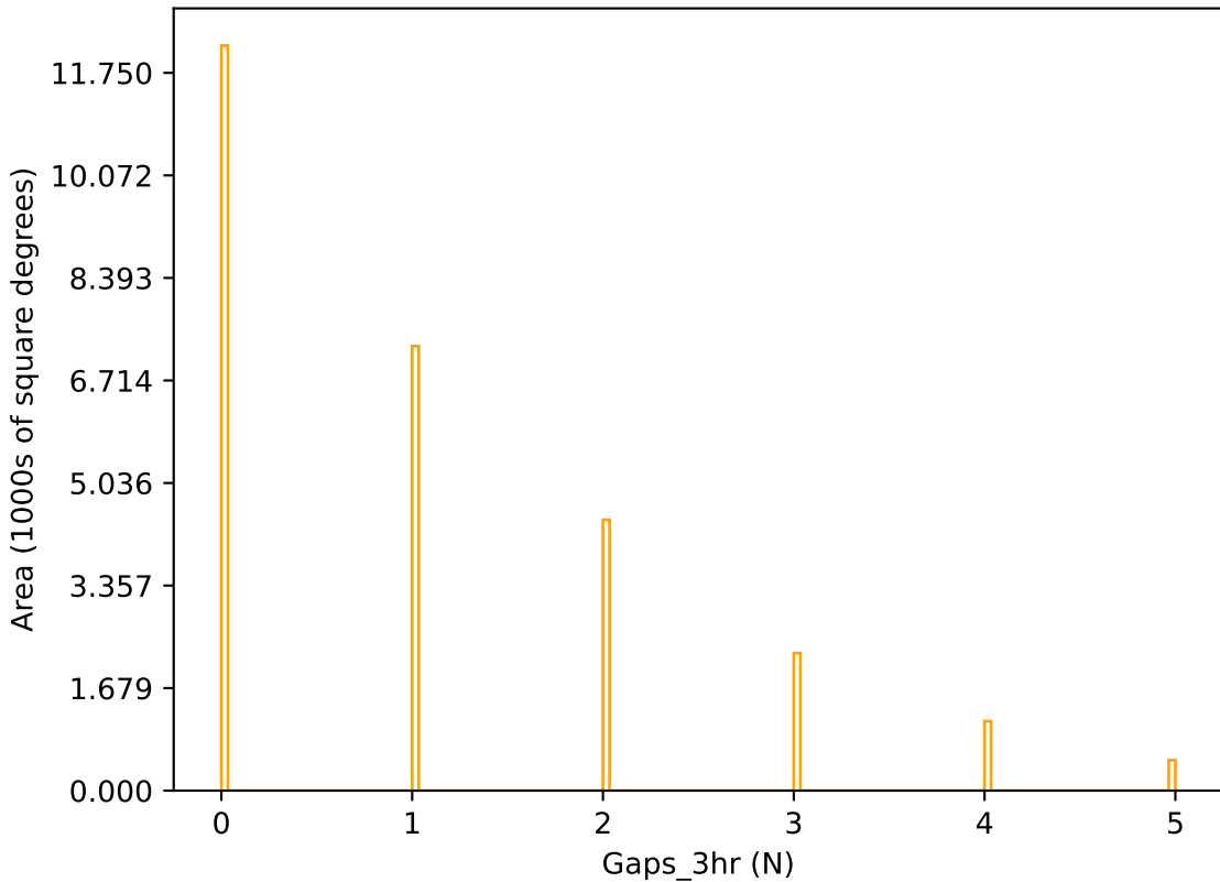
uniform_u_expt38_nscale1.1v3.4_10yrs r band: Gaps_3hr
