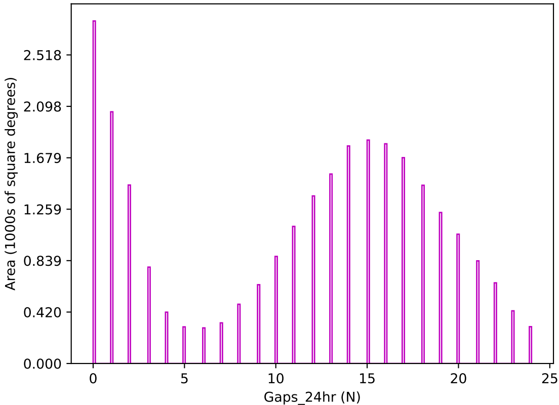
uniform_u_expt38_nscale1.1v3.4_10yrs z band: Gaps_24hr
