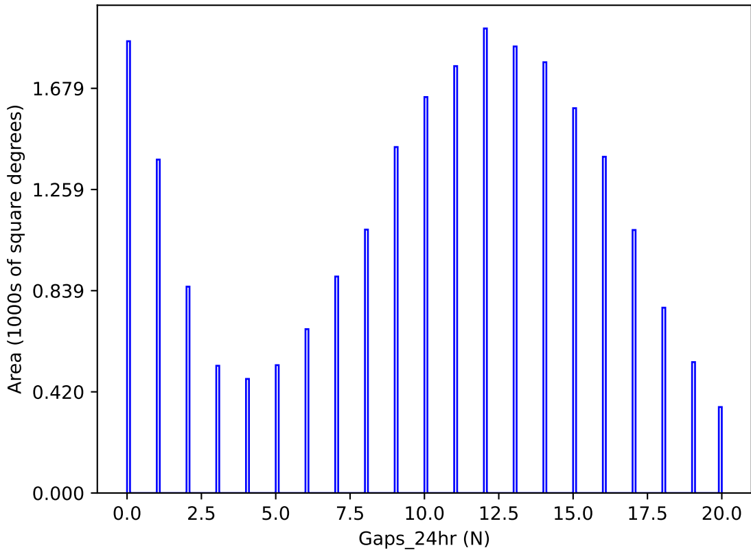
uniform_u_expt38_nscale1.1v3.4_10yrs y band: Gaps_24hr
