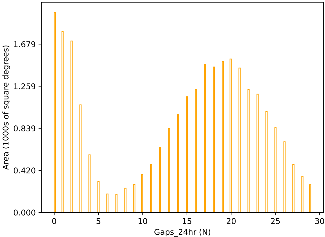
uniform_u_expt38_nscale1.1v3.4_10yrs r band: Gaps_24hr
