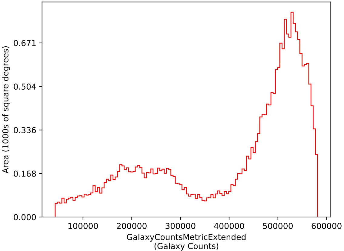
uniform_u_expt38_nscale1.1v3.4_10yrs i: GalaxyCountsMetricExtended
