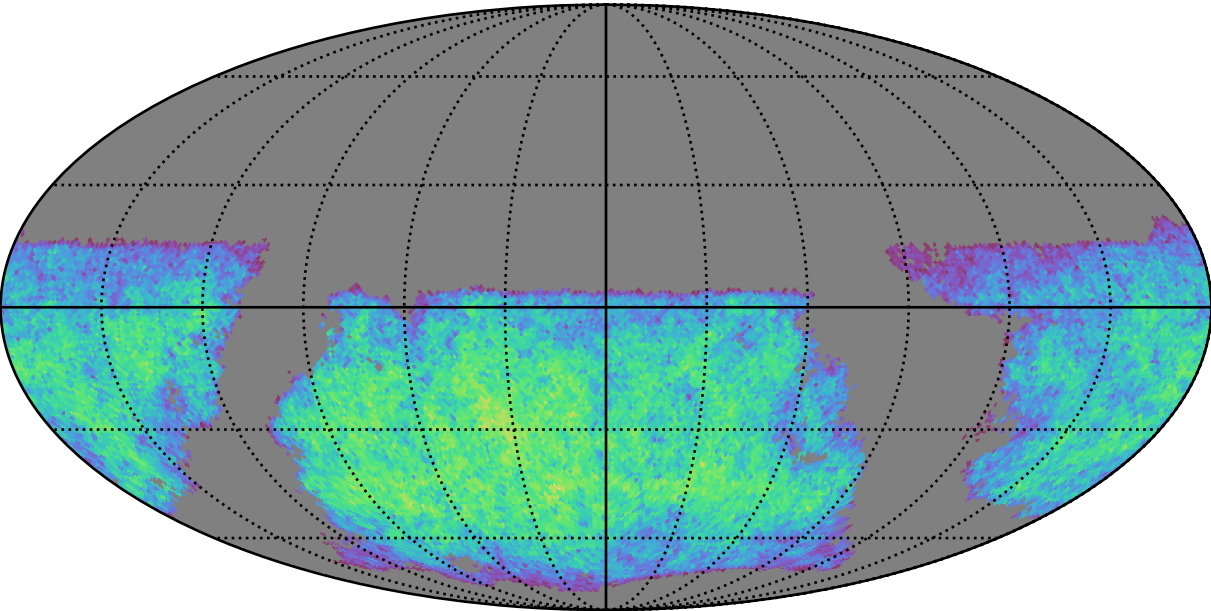
uniform_u_expt38_nscale1.1v3.4_10yrs i band non-DD year 1: ExgalM5WithCuts
