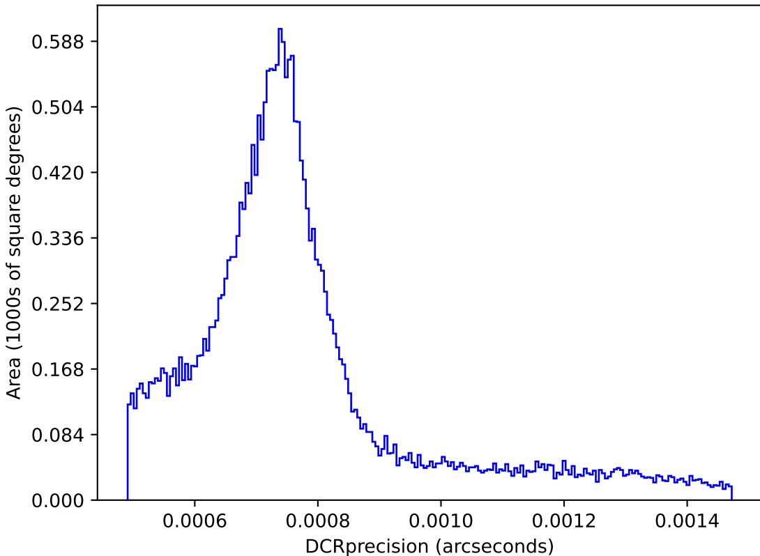
uniform_u_expt38_nscale1.1v3.4_10yrs : DCRprecision
