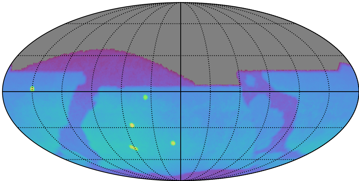
uniform_u_expt38_nscale1.1v3.4_10yrs : Brown Dwarf, L7
