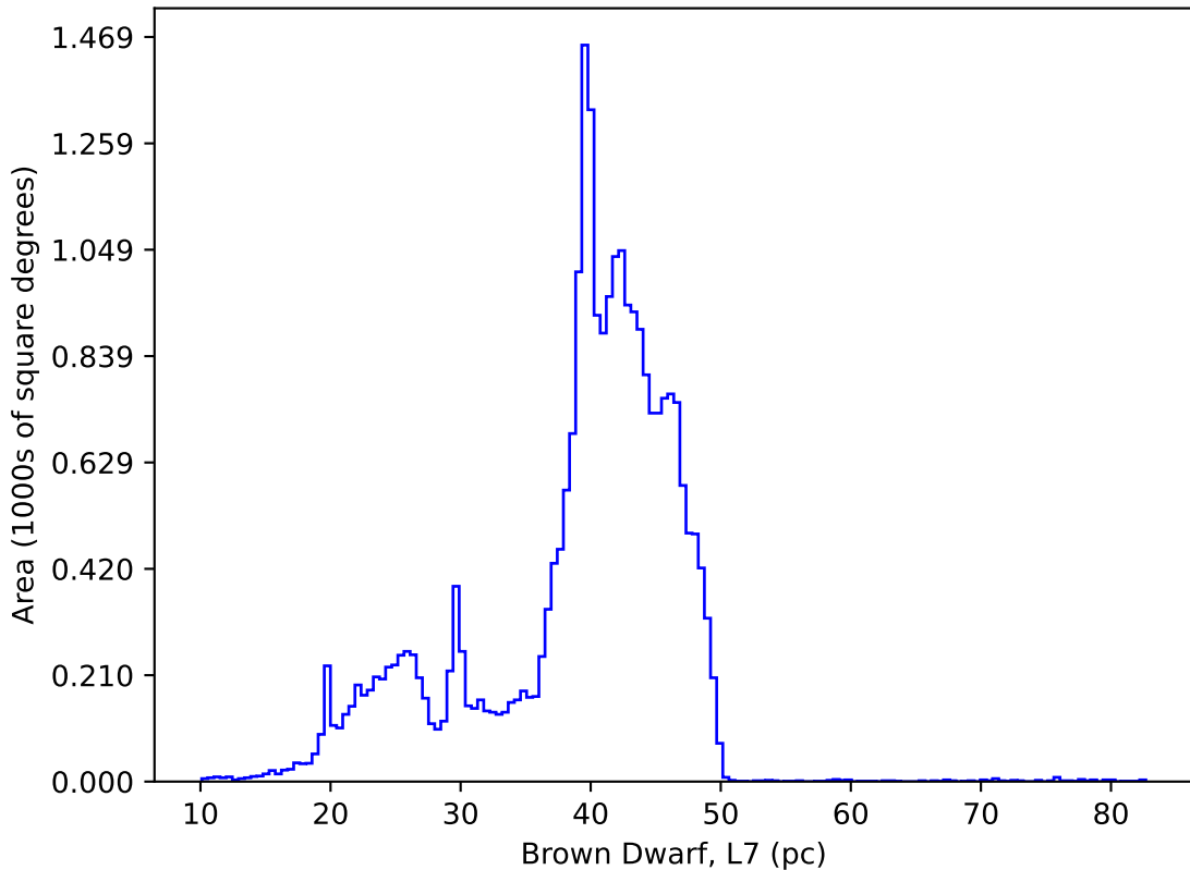
uniform_u_expt38_nscale1.1v3.4_10yrs : Brown Dwarf, L7
