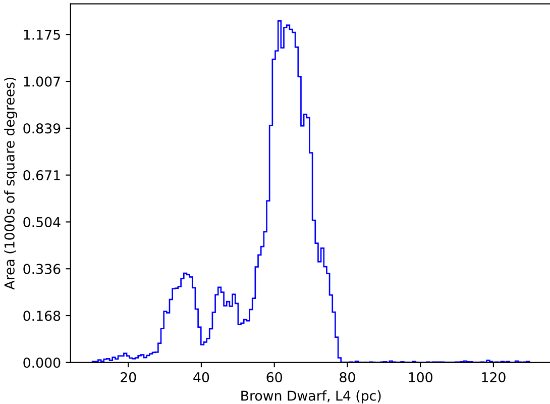
uniform_u_expt38_nscale1.1v3.4_10yrs : Brown Dwarf, L4
