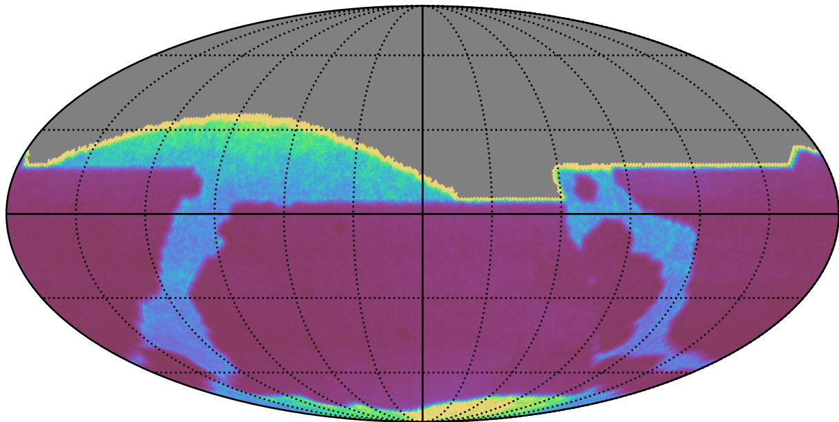
uniform_u_expt38_nscale1.1v3.4_10yrs : properMotion
